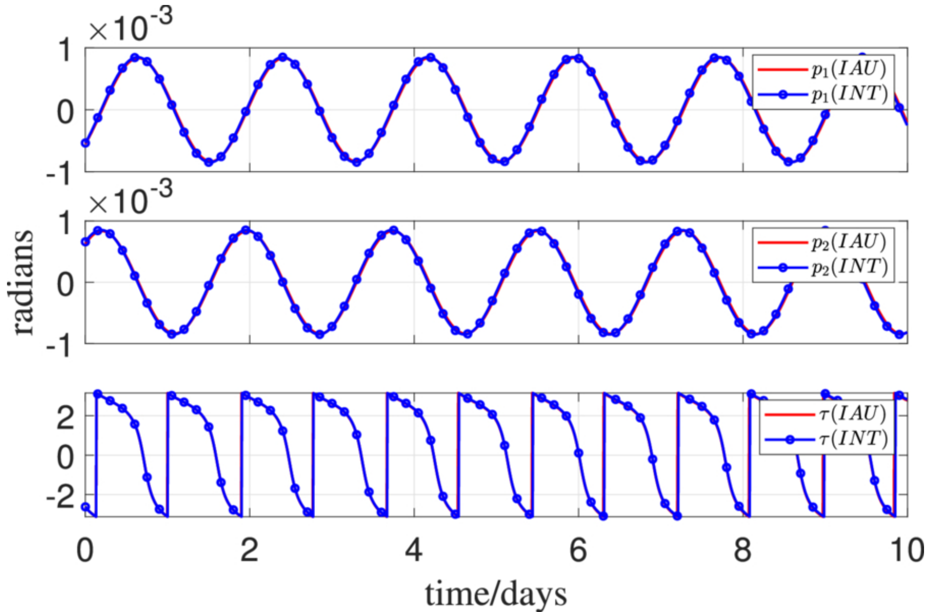
Figure 7. from Lidan Zhang et al 2025 Astron. J. 170 doi:10.3847/1538-3881/adfc54 https://dx.doi.org/10.3847/1538-3881/adfc54 © 2025. The Author(s). Published by the American Astronomical Society.
