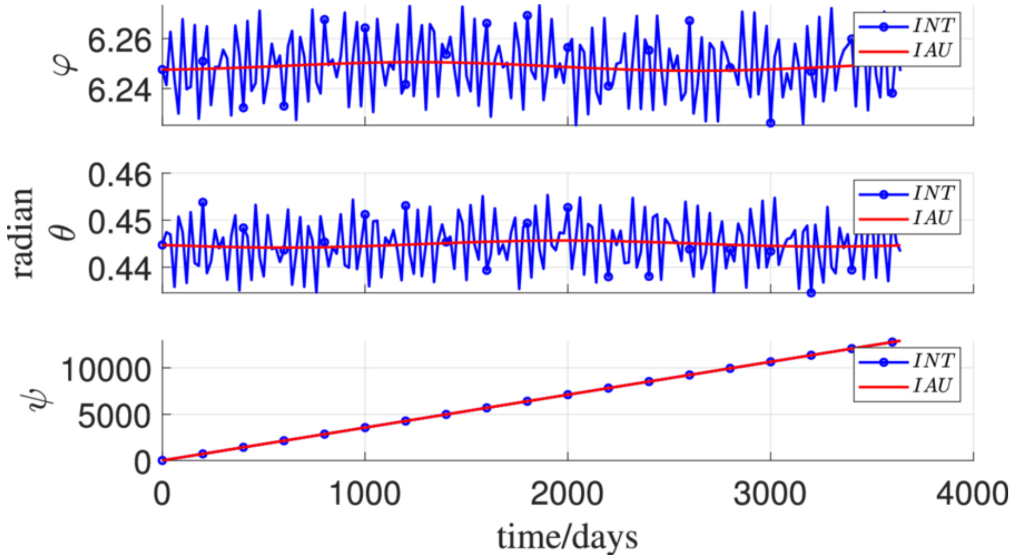
Figure 5. from Lidan Zhang et al 2025 Astron. J. 170 doi:10.3847/1538-3881/adfc54 https://dx.doi.org/10.3847/1538-3881/adfc54 © 2025. The Author(s). Published by the American Astronomical Society.
