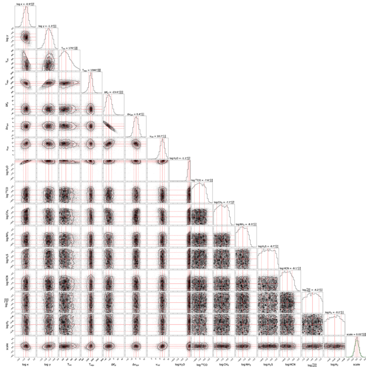
Figure 6. from Luke Finnerty et al 2025 Astron. J. 170 doi:10.3847/1538-3881/adfb71 https://dx.doi.org/10.3847/1538-3881/adfb71 © 2025. The Author(s). Published by the American Astronomical Society.
