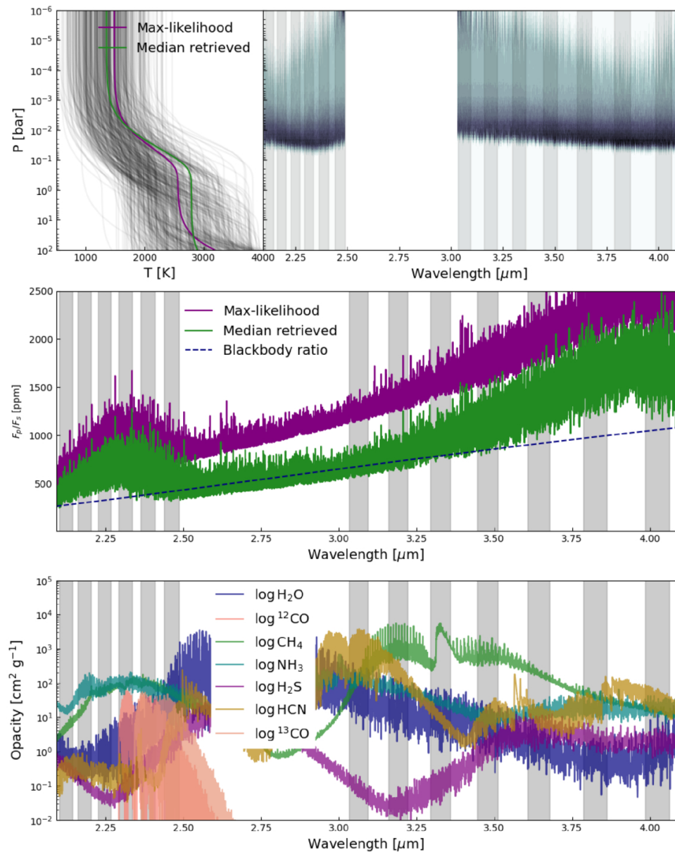
Figure 3. from Luke Finnerty et al 2025 Astron. J. 170 doi:10.3847/1538-3881/adfb71 https://dx.doi.org/10.3847/1538-3881/adfb71 © 2025. The Author(s). Published by the American Astronomical Society.
