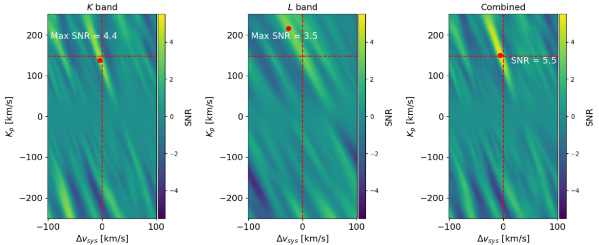
Figure 1. from Luke Finnerty et al 2025 Astron. J. 170 doi:10.3847/1538-3881/adfb71 https://dx.doi.org/10.3847/1538-3881/adfb71 © 2025. The Author(s). Published by the American Astronomical Society.
