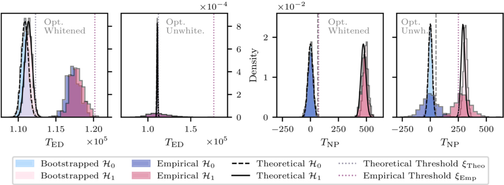
Figure 9. from Philipp A. Huber et al 2025 Astron. J. 170 doi:10.3847/1538-3881/adfb6b https://dx.doi.org/10.3847/1538-3881/adfb6b © 2025. The Author(s). Published by the American Astronomical Society.
