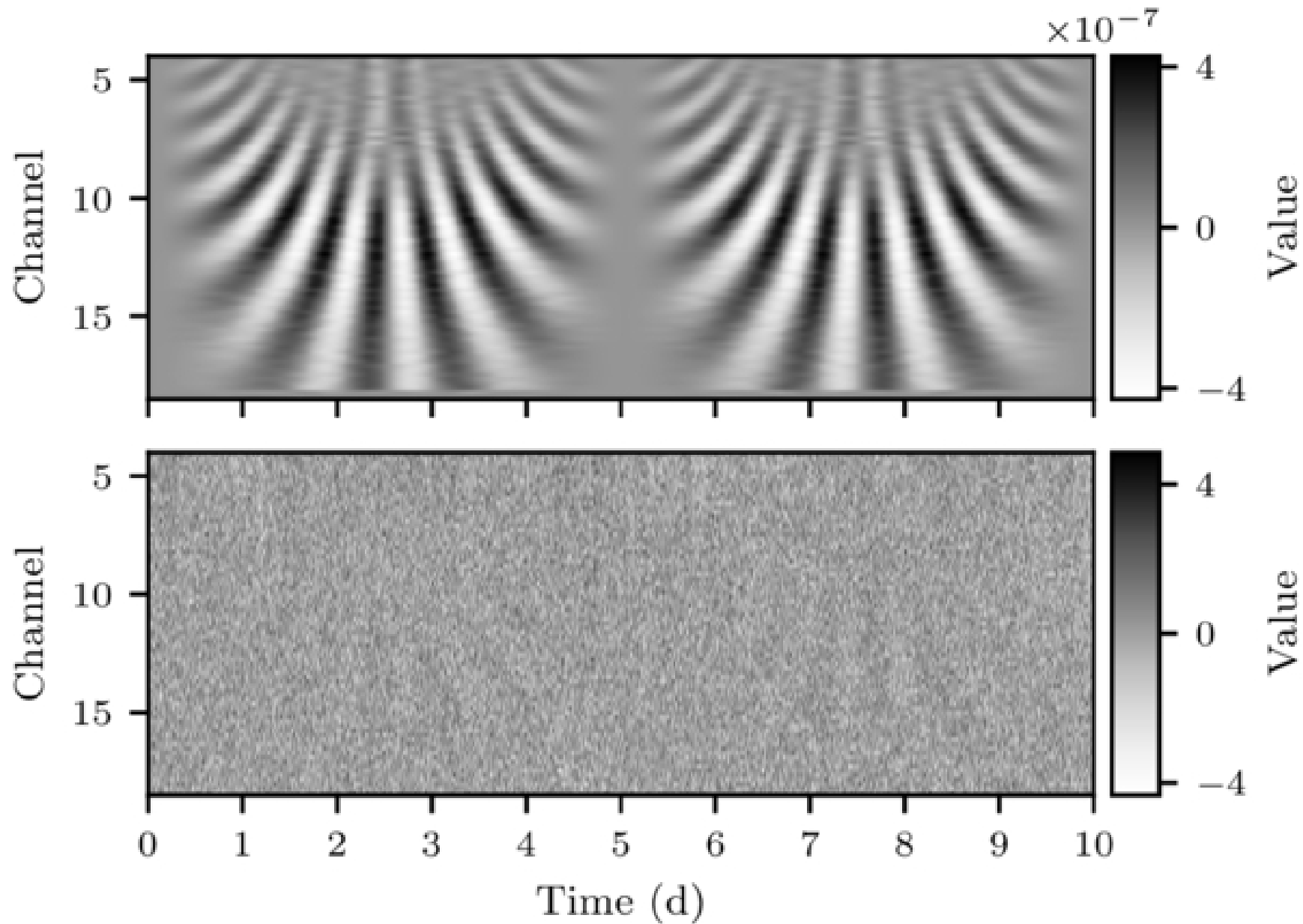
Figure 7. from Philipp A. Huber et al 2025 Astron. J. 170 doi:10.3847/1538-3881/adfb6b https://dx.doi.org/10.3847/1538-3881/adfb6b © 2025. The Author(s). Published by the American Astronomical Society.
