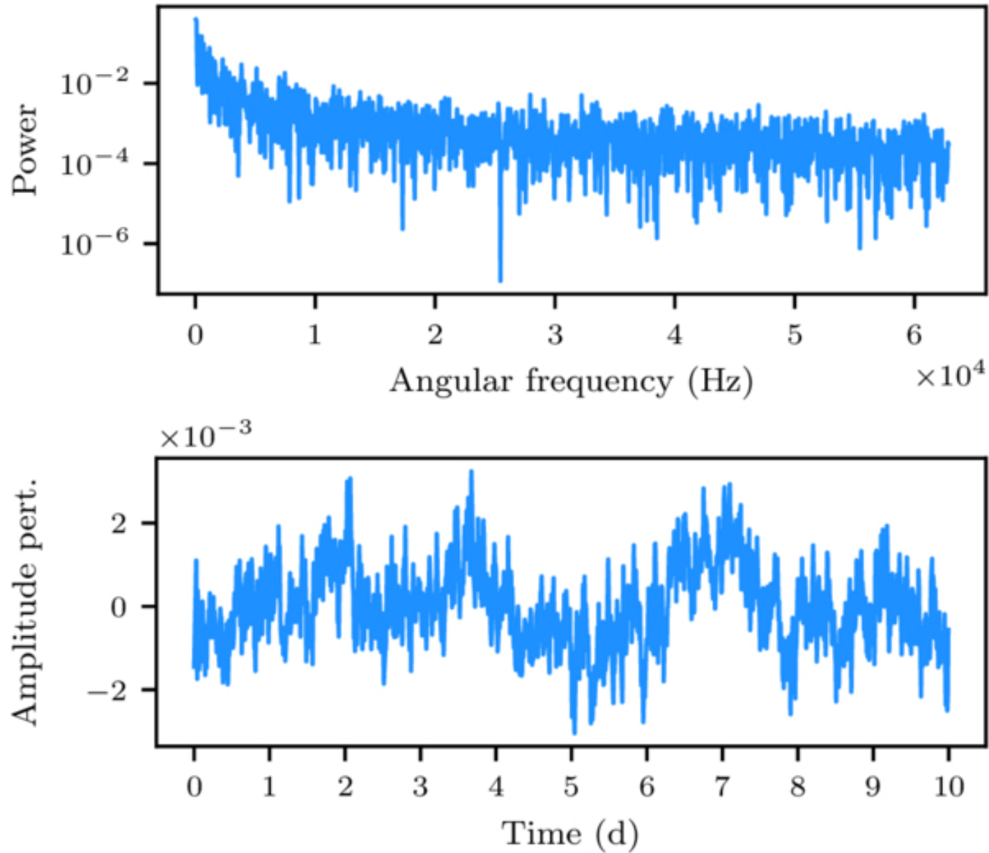
Figure 3. from Philipp A. Huber et al 2025 Astron. J. 170 doi:10.3847/1538-3881/adfb6b https://dx.doi.org/10.3847/1538-3881/adfb6b © 2025. The Author(s). Published by the American Astronomical Society.
