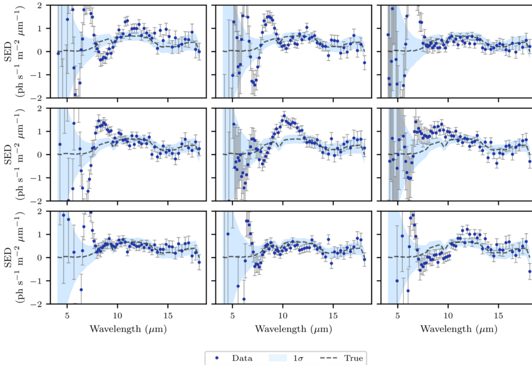
Figure 16. from Philipp A. Huber et al 2025 Astron. J. 170 doi:10.3847/1538-3881/adfb6b https://dx.doi.org/10.3847/1538-3881/adfb6b © 2025. The Author(s). Published by the American Astronomical Society.
