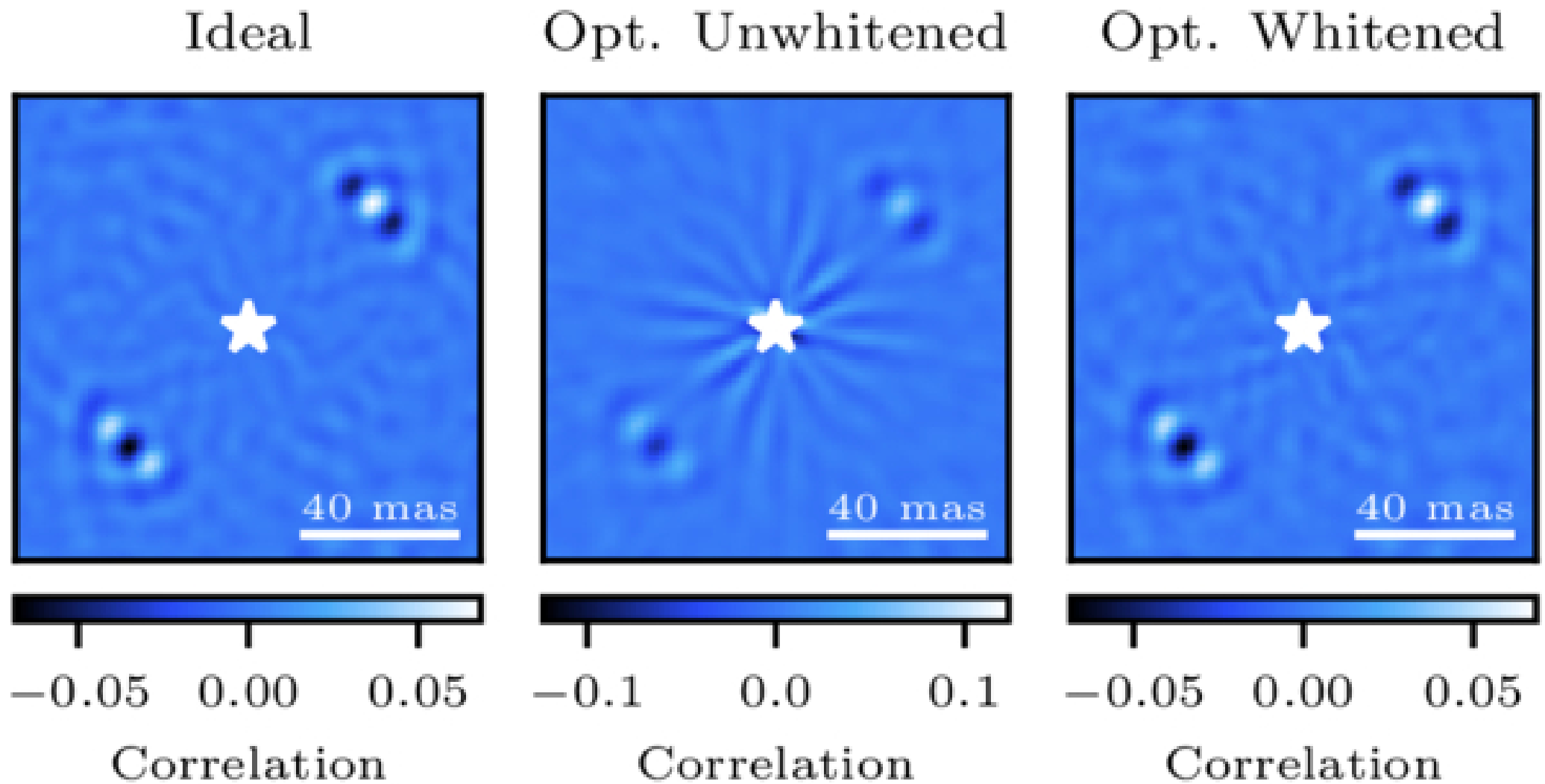
Figure 15. from Philipp A. Huber et al 2025 Astron. J. 170 doi:10.3847/1538-3881/adfb6b https://dx.doi.org/10.3847/1538-3881/adfb6b © 2025. The Author(s). Published by the American Astronomical Society.
