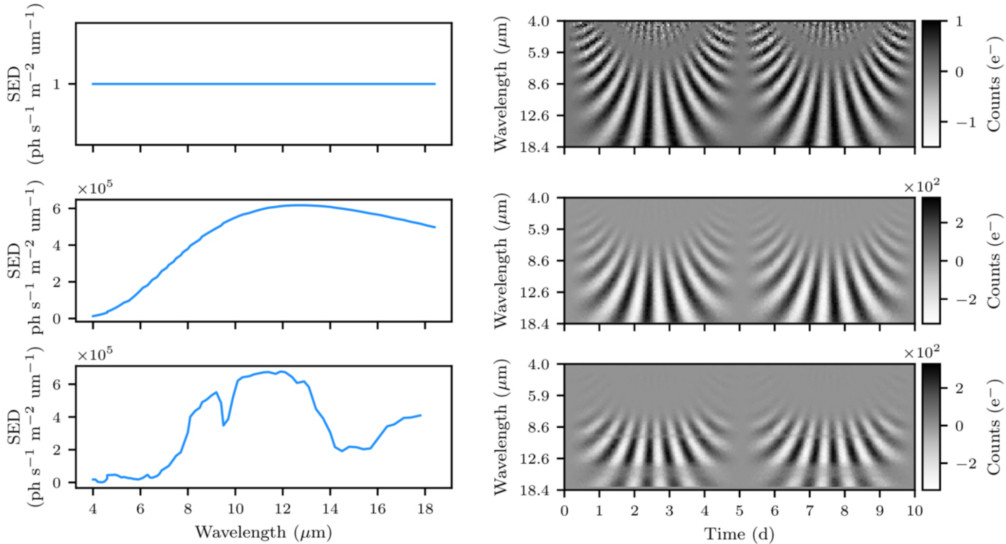
Figure 14. from Philipp A. Huber et al 2025 Astron. J. 170 doi:10.3847/1538-3881/adfb6b https://dx.doi.org/10.3847/1538-3881/adfb6b © 2025. The Author(s). Published by the American Astronomical Society.
