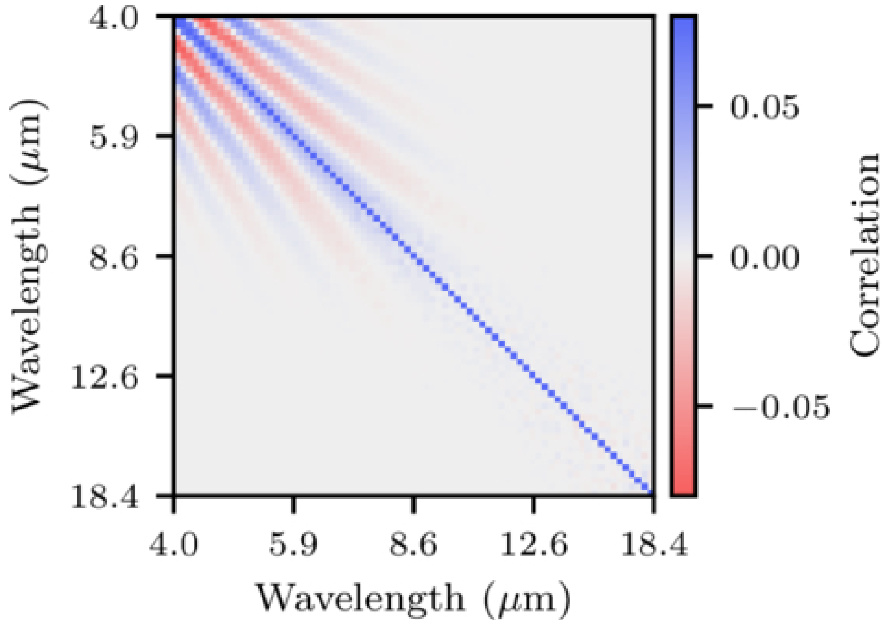
Figure 12. from Philipp A. Huber et al 2025 Astron. J. 170 doi:10.3847/1538-3881/adfb6b https://dx.doi.org/10.3847/1538-3881/adfb6b © 2025. The Author(s). Published by the American Astronomical Society.
