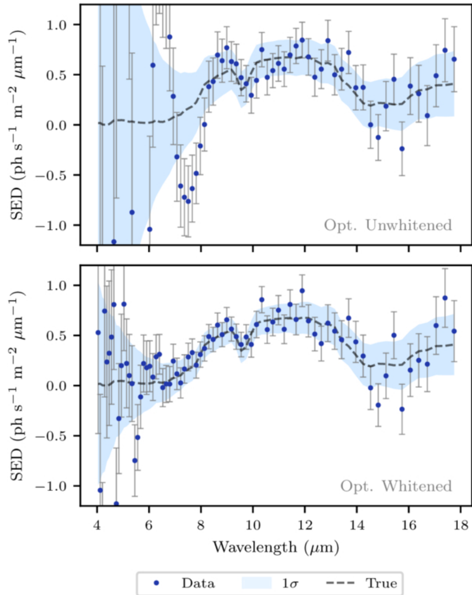
Figure 11. from Philipp A. Huber et al 2025 Astron. J. 170 doi:10.3847/1538-3881/adfb6b https://dx.doi.org/10.3847/1538-3881/adfb6b © 2025. The Author(s). Published by the American Astronomical Society.
