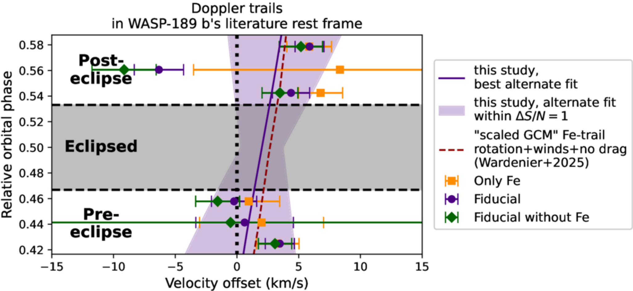
Figure 9. from Lennart van Sluijs et al 2025 Astron. J. 170 doi:10.3847/1538-3881/adfb61 https://dx.doi.org/10.3847/1538-3881/adfb61 © 2025. The Author(s). Published by the American Astronomical Society.
