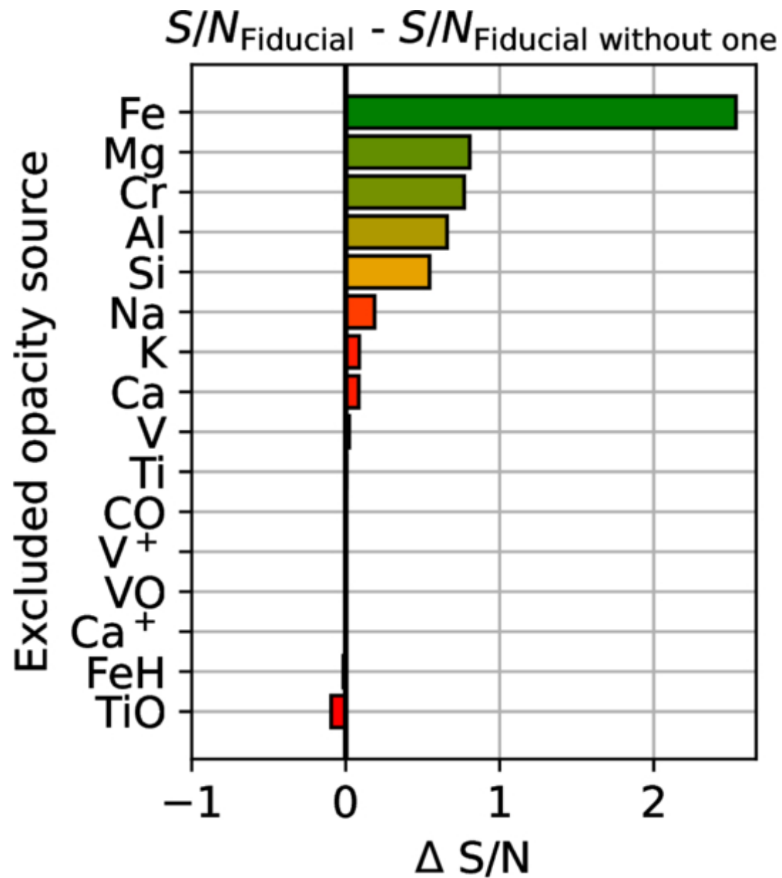
Figure 7. from Lennart van Sluijs et al 2025 Astron. J. 170 doi:10.3847/1538-3881/adfb61 https://dx.doi.org/10.3847/1538-3881/adfb61 © 2025. The Author(s). Published by the American Astronomical Society.
