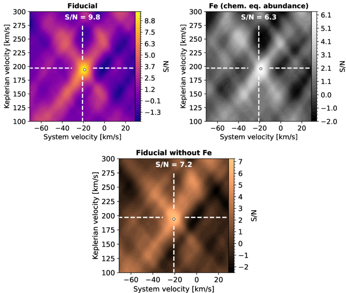
Figure 6. from Lennart van Sluijs et al 2025 Astron. J. 170 doi:10.3847/1538-3881/adfb61 https://dx.doi.org/10.3847/1538-3881/adfb61 © 2025. The Author(s). Published by the American Astronomical Society.
