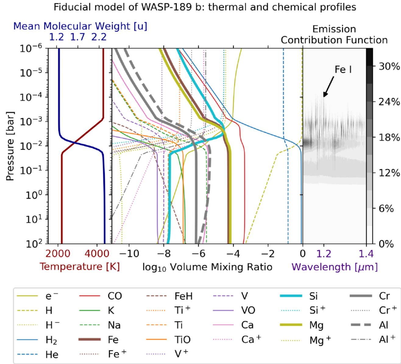
Figure 4. from Lennart van Sluijs et al 2025 Astron. J. 170 doi:10.3847/1538-3881/adfb61 https://dx.doi.org/10.3847/1538-3881/adfb61 © 2025. The Author(s). Published by the American Astronomical Society.
