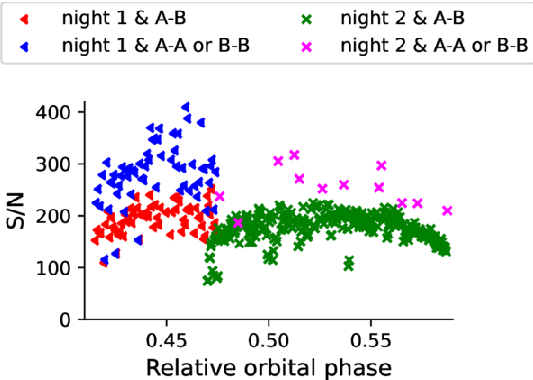
Figure 3. from Lennart van Sluijs et al 2025 Astron. J. 170 doi:10.3847/1538-3881/adfb61 https://dx.doi.org/10.3847/1538-3881/adfb61 © 2025. The Author(s). Published by the American Astronomical Society.
