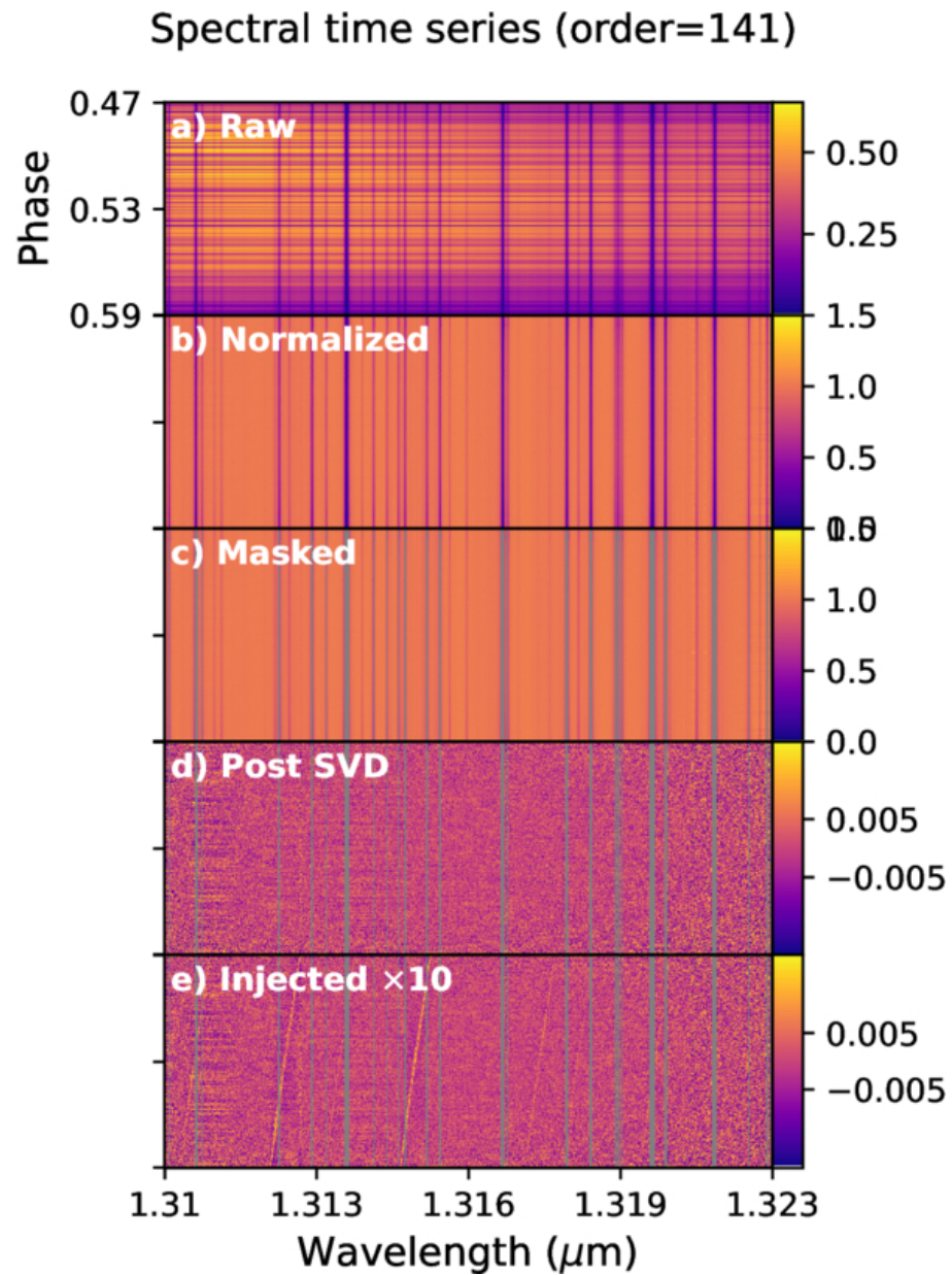
Figure 2. from Lennart van Sluijs et al 2025 Astron. J. 170 doi:10.3847/1538-3881/adfb61 https://dx.doi.org/10.3847/1538-3881/adfb61 © 2025. The Author(s). Published by the American Astronomical Society.
