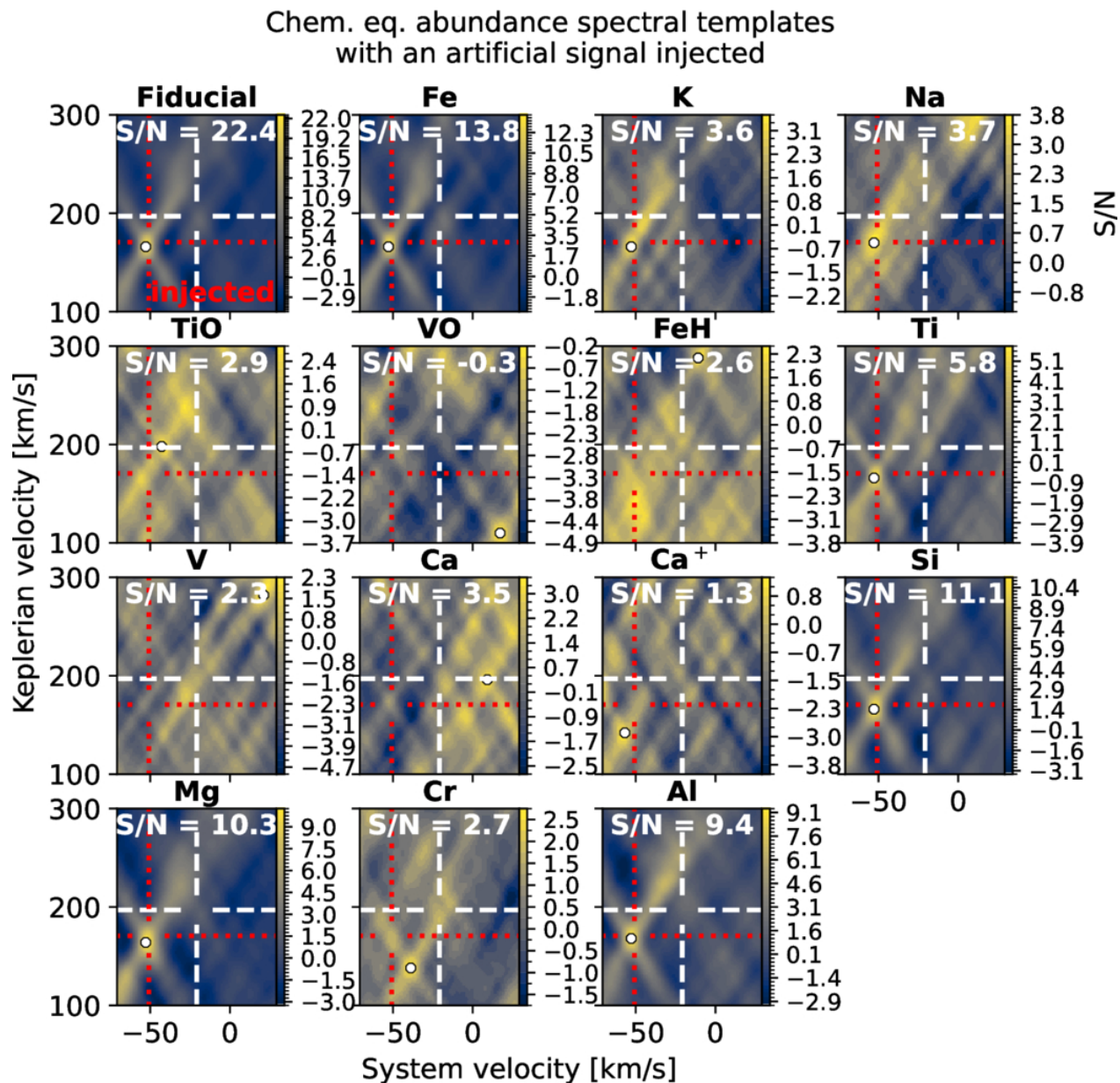
Figure 17. from Lennart van Sluijs et al 2025 Astron. J. 170 doi:10.3847/1538-3881/adfb61 https://dx.doi.org/10.3847/1538-3881/adfb61 © 2025. The Author(s). Published by the American Astronomical Society.
