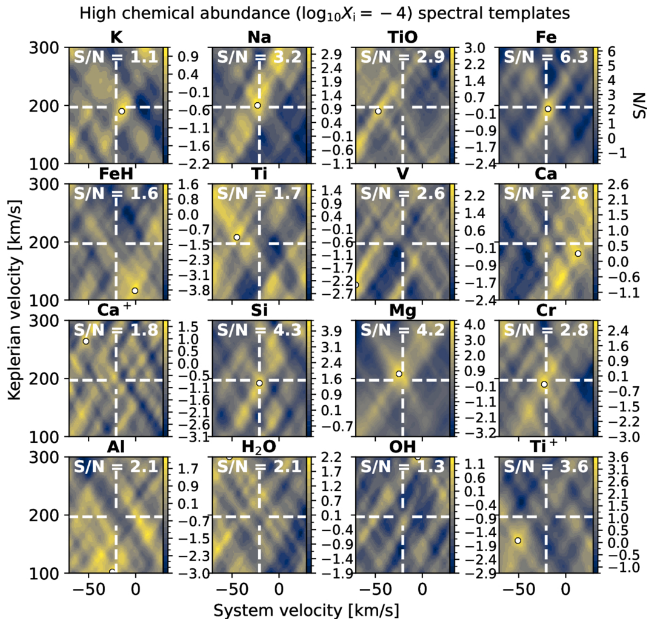
Figure 16. from Lennart van Sluijs et al 2025 Astron. J. 170 doi:10.3847/1538-3881/adfb61 https://dx.doi.org/10.3847/1538-3881/adfb61 © 2025. The Author(s). Published by the American Astronomical Society.
