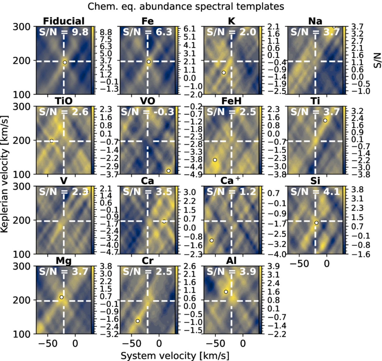
Figure 15. from Lennart van Sluijs et al 2025 Astron. J. 170 doi:10.3847/1538-3881/adfb61 https://dx.doi.org/10.3847/1538-3881/adfb61 © 2025. The Author(s). Published by the American Astronomical Society.
