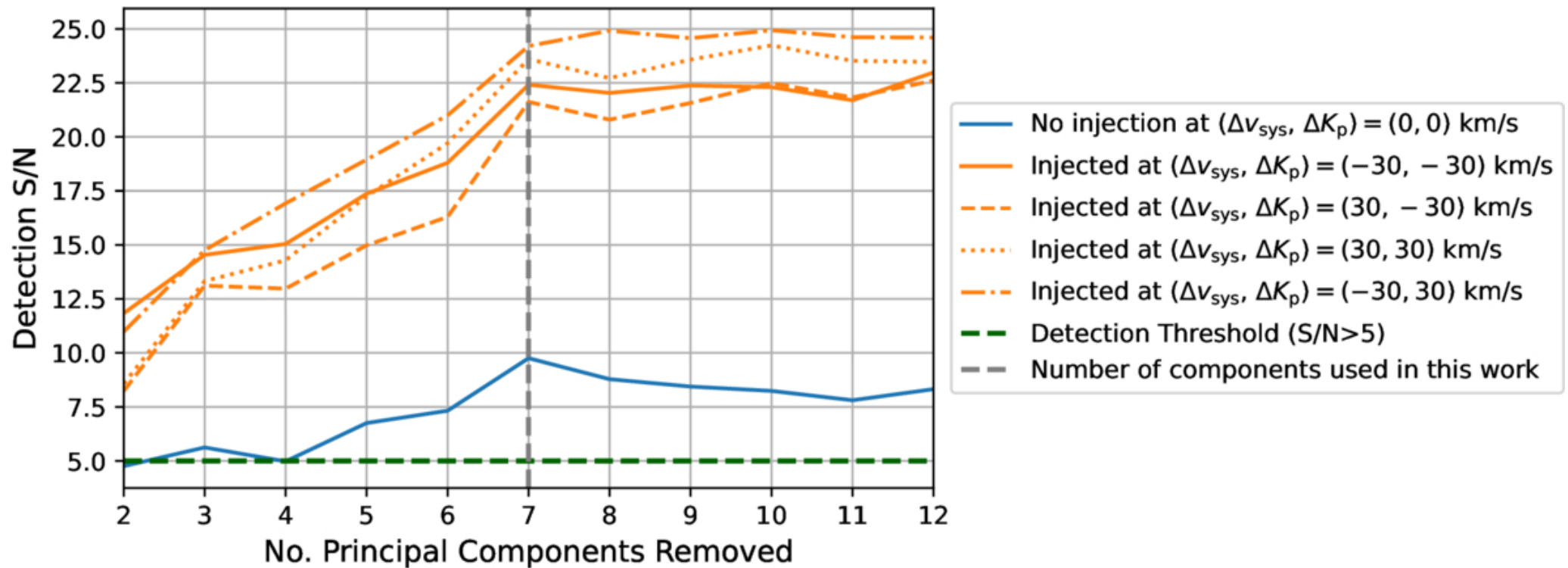
Figure 12. from Lennart van Sluijs et al 2025 Astron. J. 170 doi:10.3847/1538-3881/adfb61 https://dx.doi.org/10.3847/1538-3881/adfb61 © 2025. The Author(s). Published by the American Astronomical Society.
