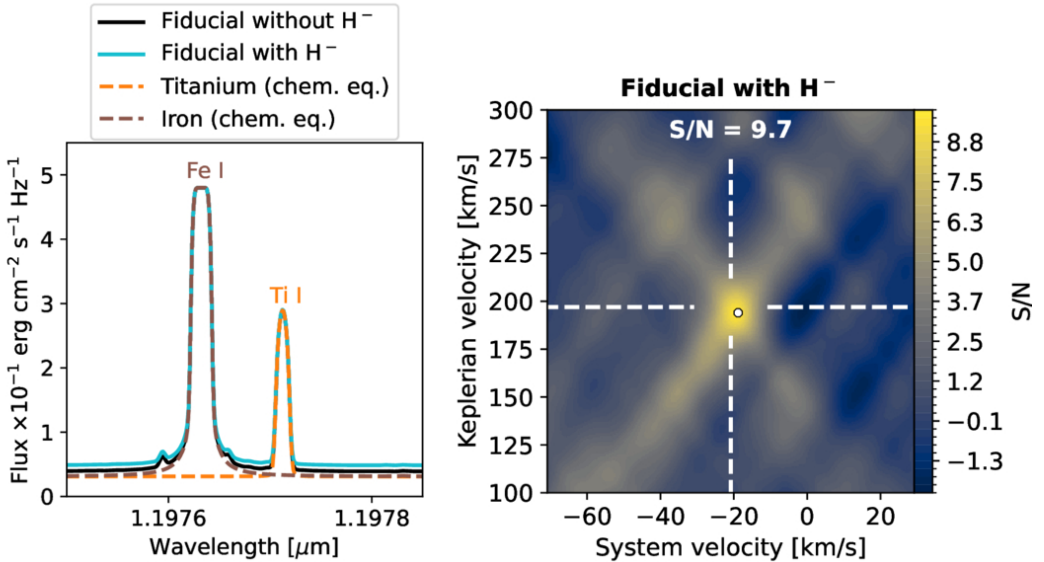
Figure 11. from Lennart van Sluijs et al 2025 Astron. J. 170 doi:10.3847/1538-3881/adfb61 https://dx.doi.org/10.3847/1538-3881/adfb61 © 2025. The Author(s). Published by the American Astronomical Society.
