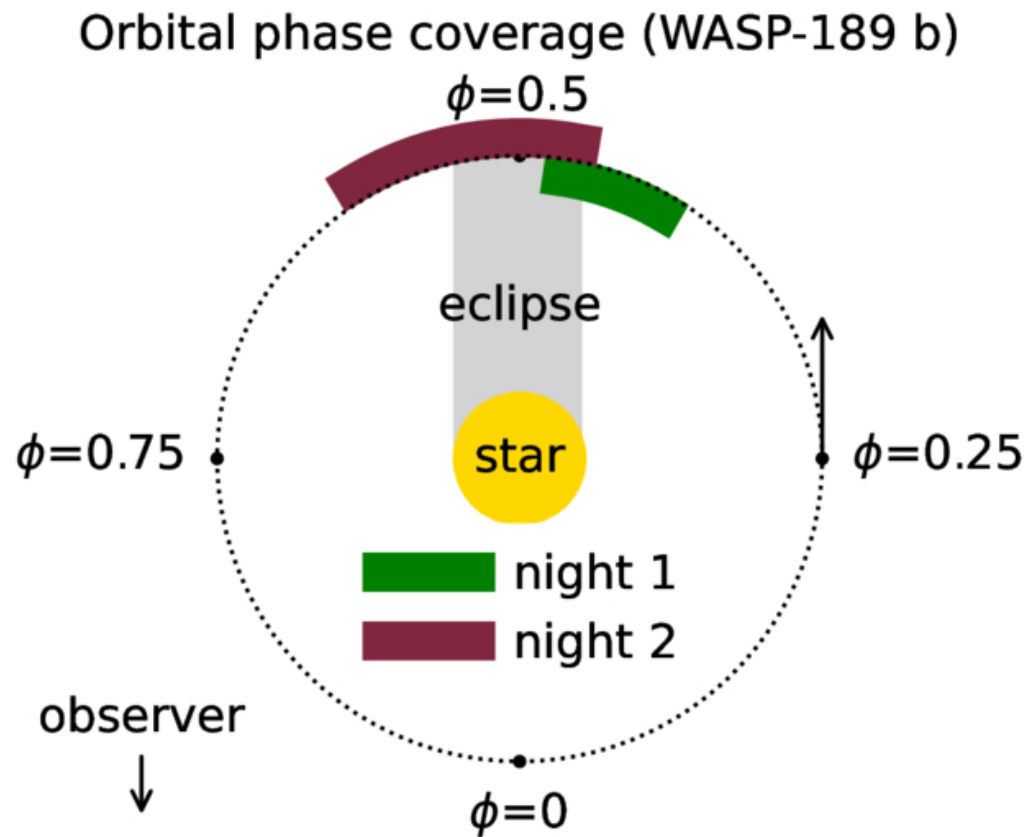
Figure 1. from Lennart van Sluijs et al 2025 Astron. J. 170 doi:10.3847/1538-3881/adfb61 https://dx.doi.org/10.3847/1538-3881/adfb61 © 2025. The Author(s). Published by the American Astronomical Society.
