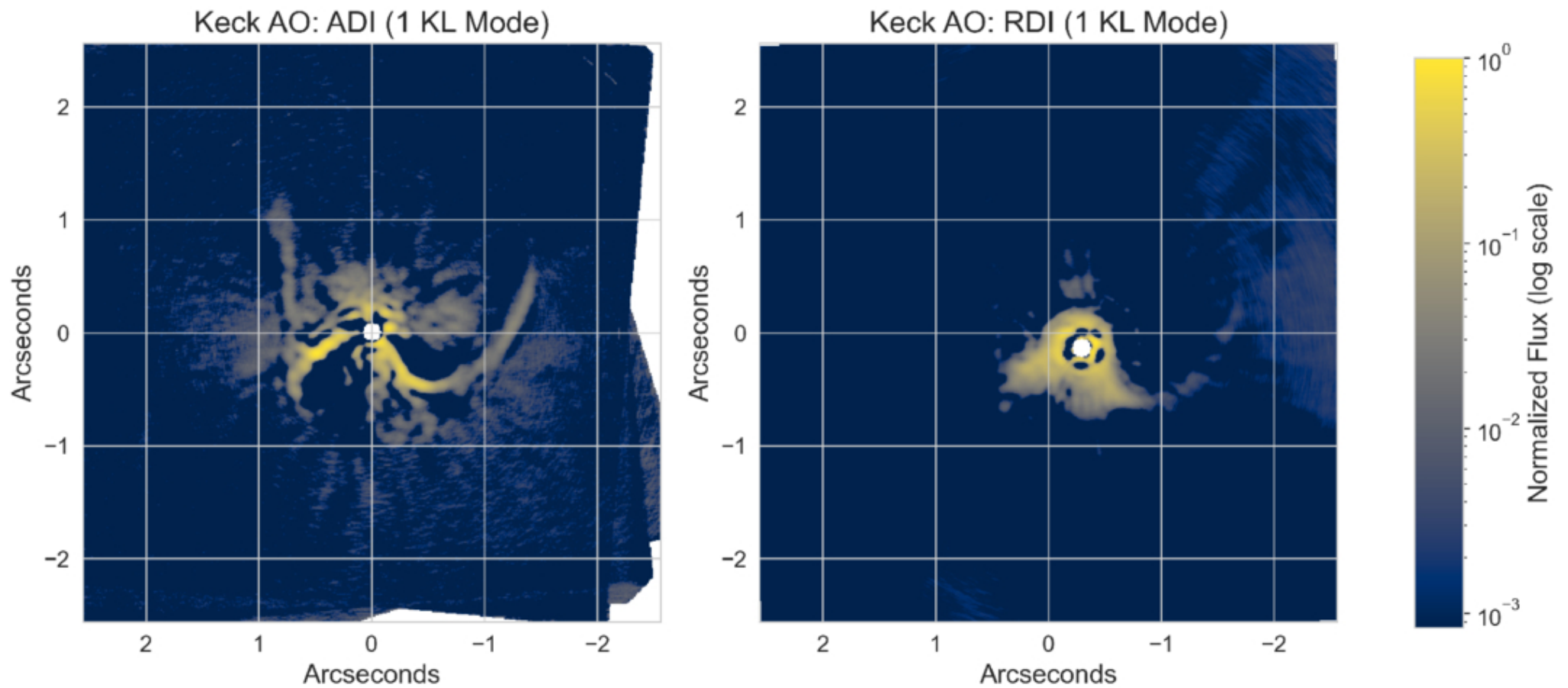
Figure 8. from John D. Monnier et al 2025 Astron. J. 170 doi:10.3847/1538-3881/adfa03 https://dx.doi.org/10.3847/1538-3881/adfa03 © 2025. The Author(s). Published by the American Astronomical Society.
