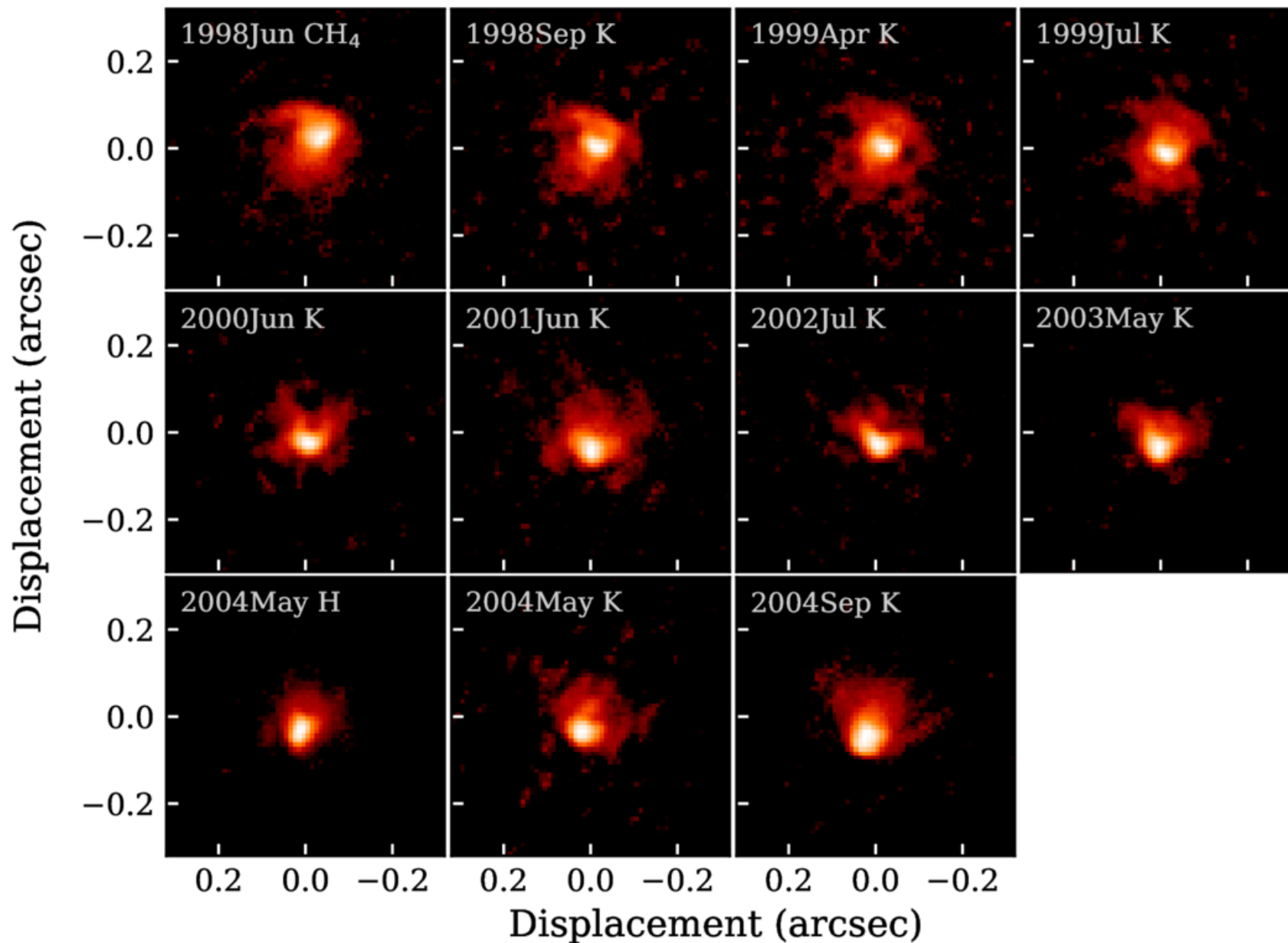
Figure 7. from John D. Monnier et al 2025 Astron. J. 170 doi:10.3847/1538-3881/adfa03 https://dx.doi.org/10.3847/1538-3881/adfa03 © 2025. The Author(s). Published by the American Astronomical Society.
