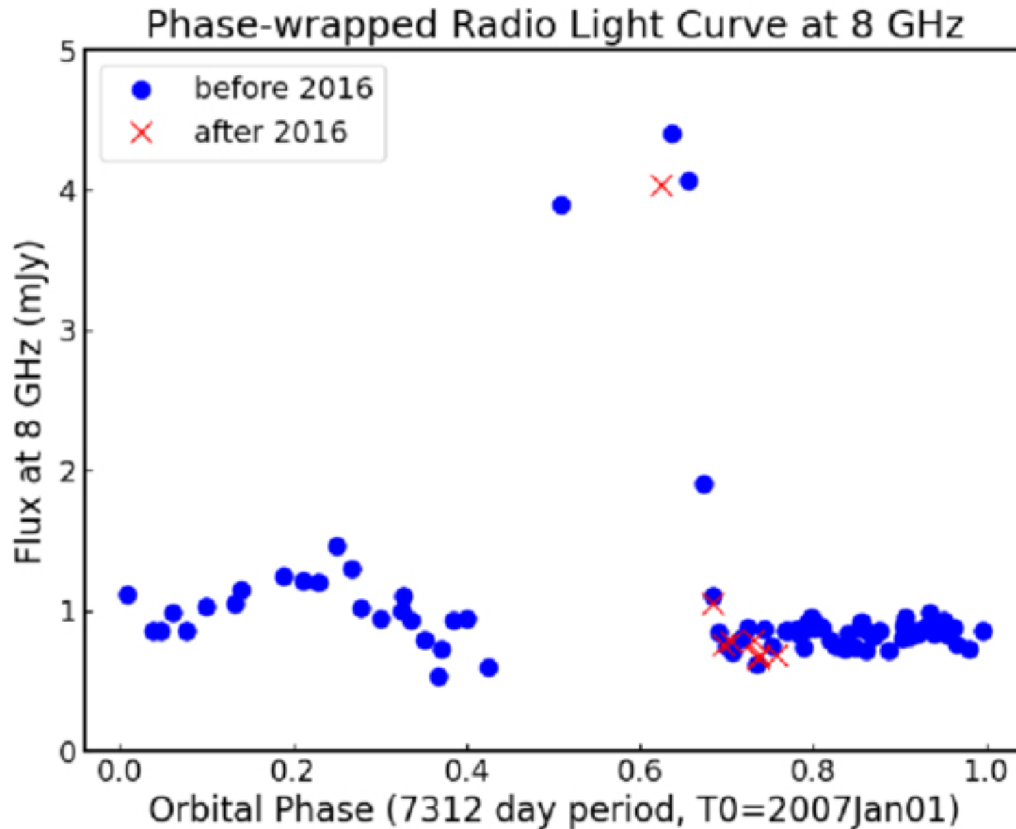
Figure 6. from John D. Monnier et al 2025 Astron. J. 170 doi:10.3847/1538-3881/adfa03 https://dx.doi.org/10.3847/1538-3881/adfa03 © 2025. The Author(s). Published by the American Astronomical Society.
