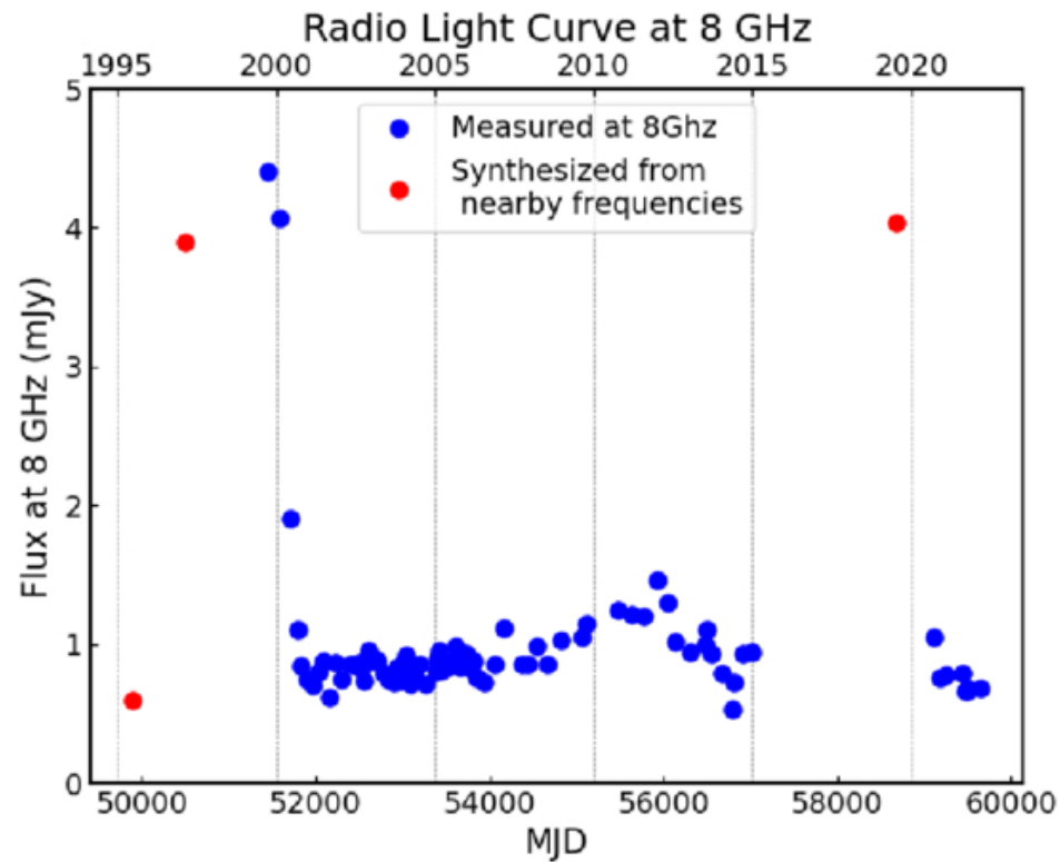
Figure 5. from John D. Monnier et al 2025 Astron. J. 170 doi:10.3847/1538-3881/adfa03 https://dx.doi.org/10.3847/1538-3881/adfa03 © 2025. The Author(s). Published by the American Astronomical Society.
