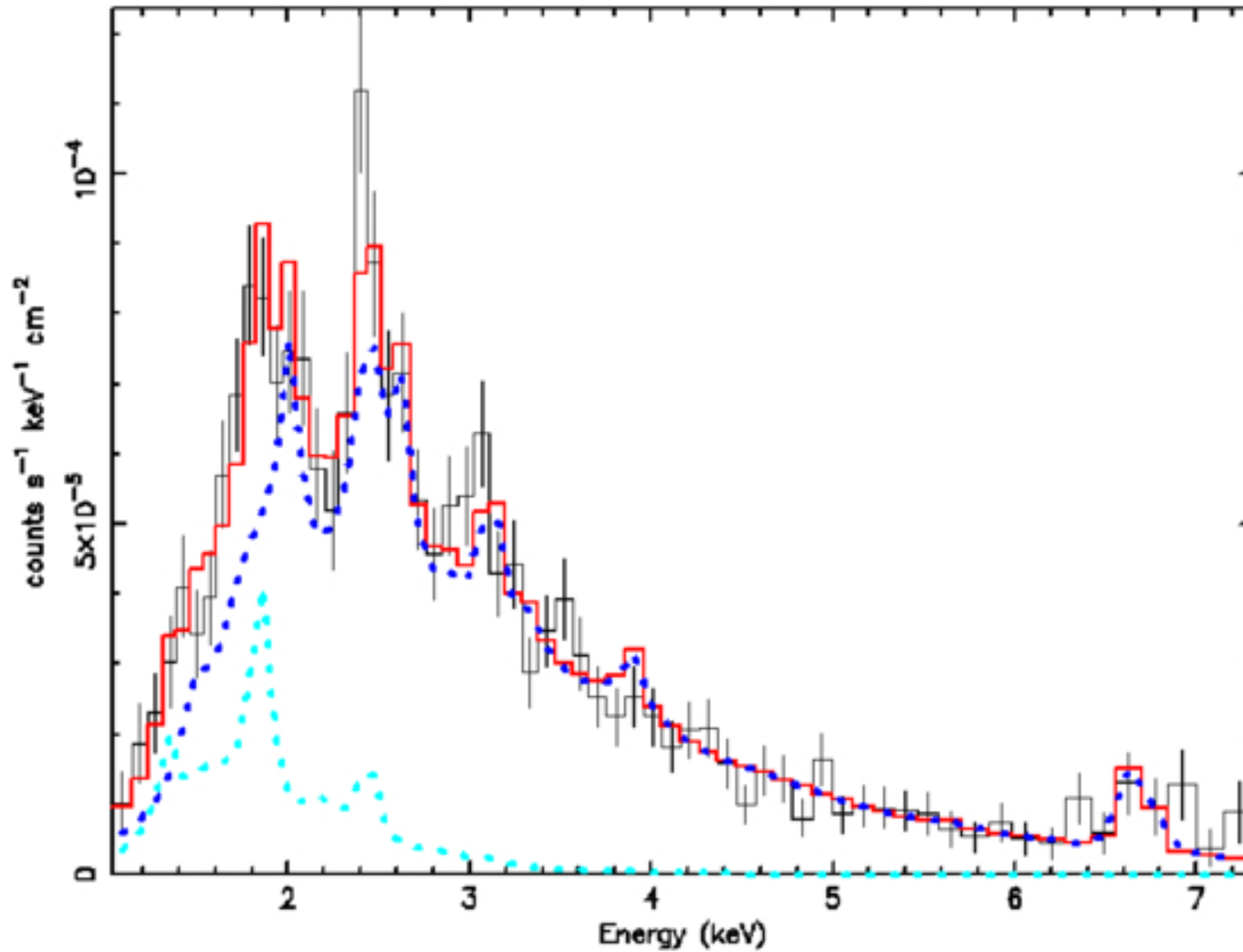
Figure 4. from John D. Monnier et al 2025 Astron. J. 170 doi:10.3847/1538-3881/adfa03 https://dx.doi.org/10.3847/1538-3881/adfa03 © 2025. The Author(s). Published by the American Astronomical Society.
