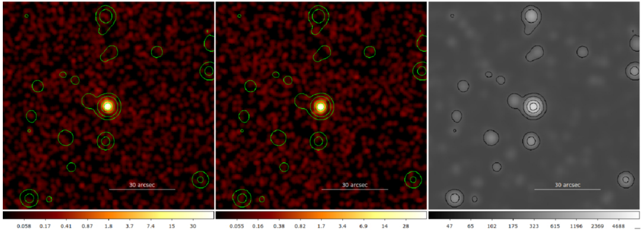
Figure 2. from John D. Monnier et al 2025 Astron. J. 170 doi:10.3847/1538-3881/adfa03 https://dx.doi.org/10.3847/1538-3881/adfa03 © 2025. The Author(s). Published by the American Astronomical Society.
