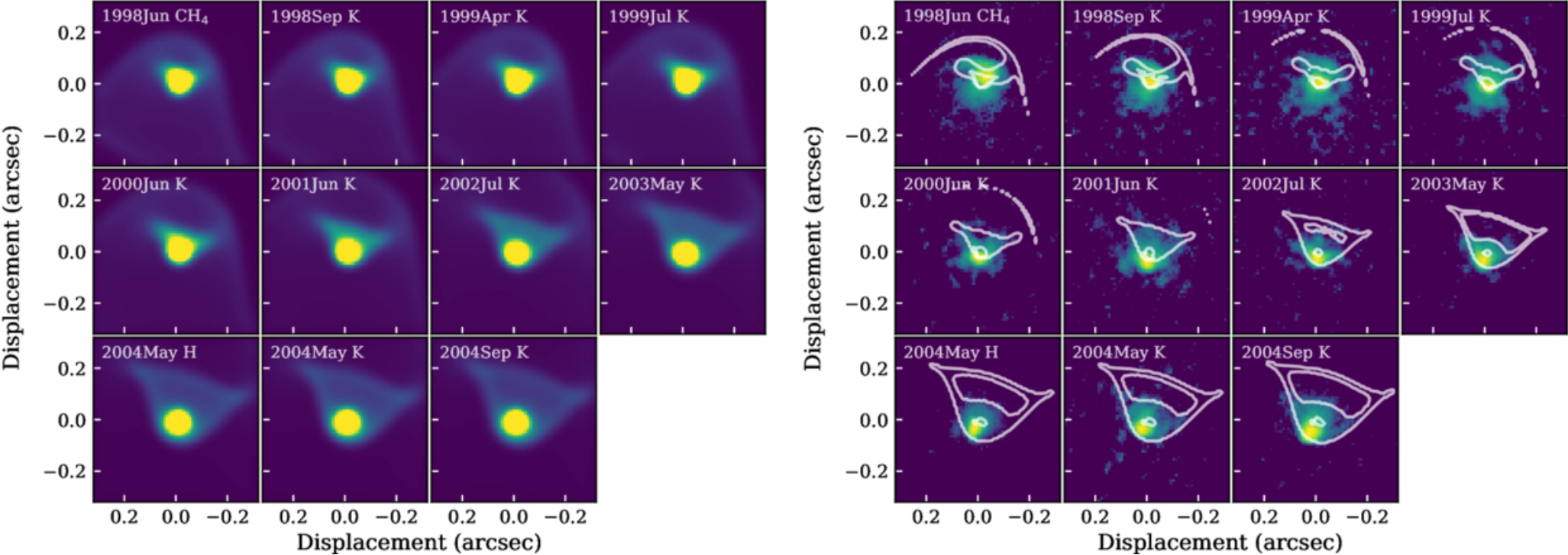
Figure 10. from John D. Monnier et al 2025 Astron. J. 170 doi:10.3847/1538-3881/adfa03 https://dx.doi.org/10.3847/1538-3881/adfa03 © 2025. The Author(s). Published by the American Astronomical Society.
