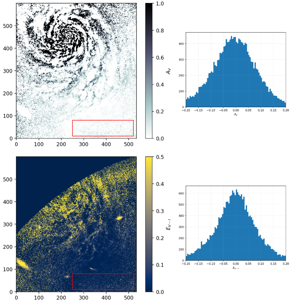
Figure 13. from Clayton D. Robertson et al 2025 Astron. J. 170 doi:10.3847/1538-3881/adf6aa https://dx.doi.org/10.3847/1538-3881/adf6aa © 2025. The Author(s). Published by the American Astronomical Society.
