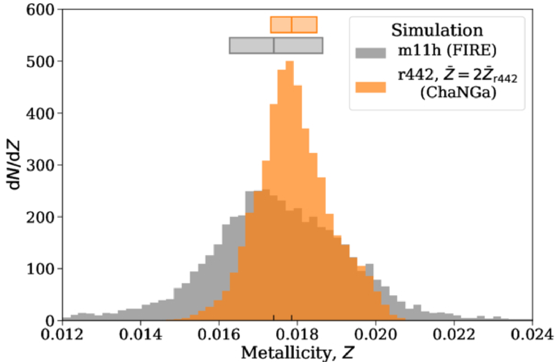
Figure 8. from Tom Wagg et al 2025 Astron. J. 170 doi:10.3847/1538-3881/adf55e https://dx.doi.org/10.3847/1538-3881/adf55e © 2025. The Author(s). Published by the American Astronomical Society.
