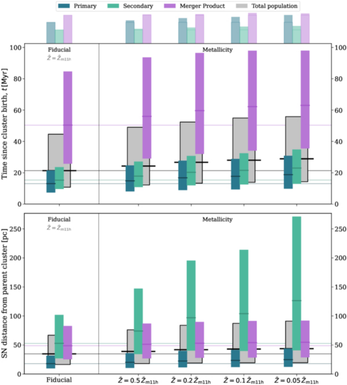
Figure 6. from Tom Wagg et al 2025 Astron. J. 170 doi:10.3847/1538-3881/adf55e https://dx.doi.org/10.3847/1538-3881/adf55e © 2025. The Author(s). Published by the American Astronomical Society.
