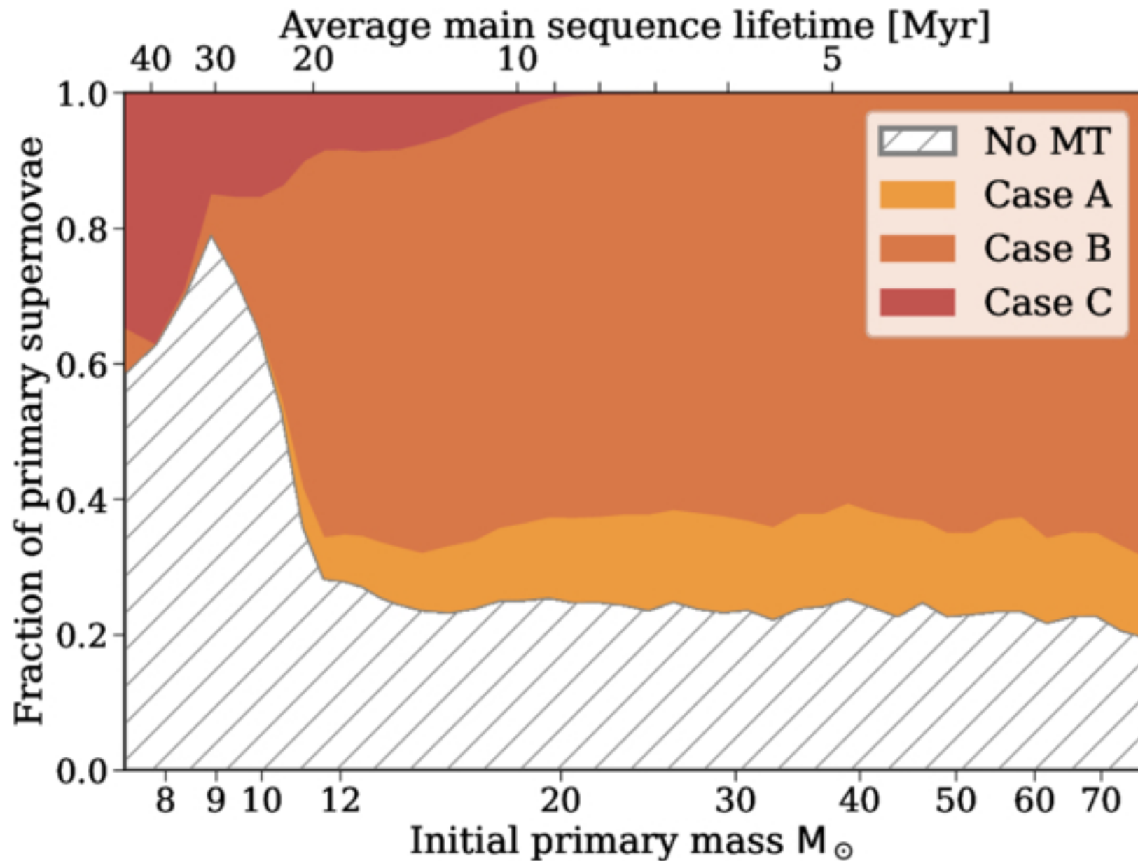
Figure 2. from Tom Wagg et al 2025 Astron. J. 170 doi:10.3847/1538-3881/adf55e https://dx.doi.org/10.3847/1538-3881/adf55e © 2025. The Author(s). Published by the American Astronomical Society.
