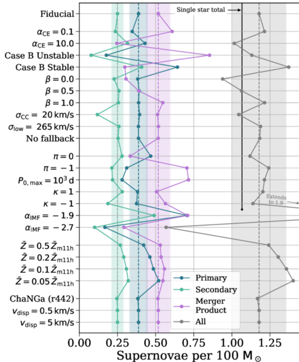
Figure 14. from Tom Wagg et al 2025 Astron. J. 170 doi:10.3847/1538-3881/adf55e https://dx.doi.org/10.3847/1538-3881/adf55e © 2025. The Author(s). Published by the American Astronomical Society.
