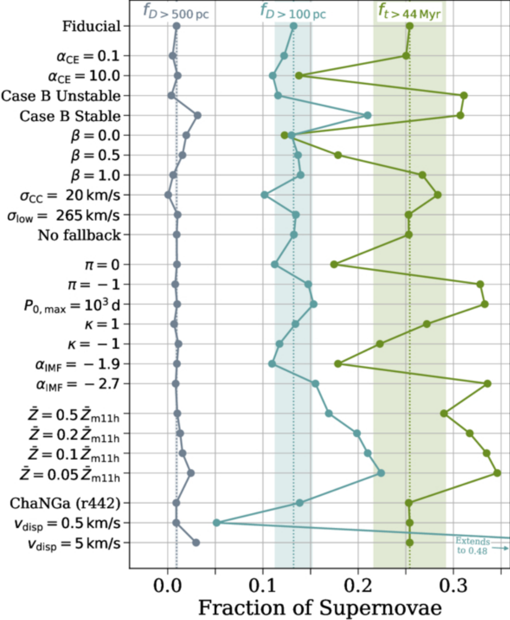
Figure 13. from Tom Wagg et al 2025 Astron. J. 170 doi:10.3847/1538-3881/adf55e https://dx.doi.org/10.3847/1538-3881/adf55e © 2025. The Author(s). Published by the American Astronomical Society.
