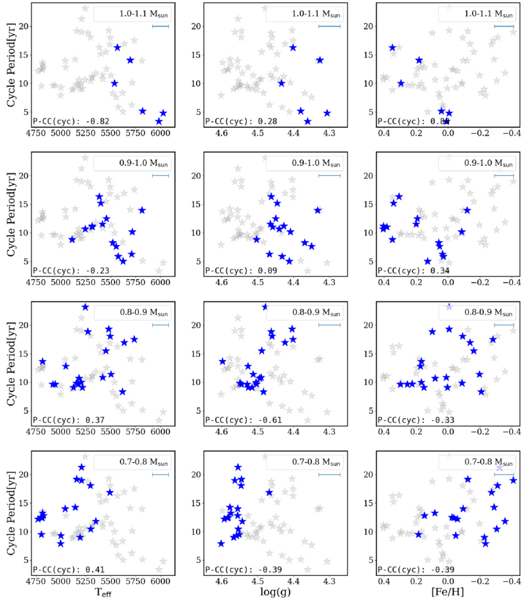
Figure 7. from Howard Isaacson et al 2025 Astron. J. 170 doi:10.3847/1538-3881/adf2a8 https://dx.doi.org/10.3847/1538-3881/adf2a8 © 2025. The Author(s). Published by the American Astronomical Society.
