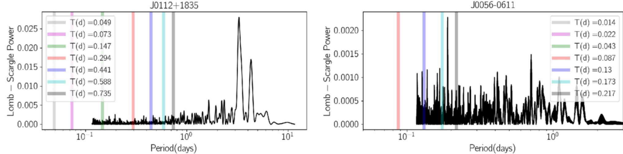
Figure 7. from Sedighe Sajadian and Aref Asadi 2025 Astron. J. 170 doi:10.3847/1538-3881/adf0f6 https://dx.doi.org/10.3847/1538-3881/adf0f6 © 2025. The Author(s). Published by the American Astronomical Society.
