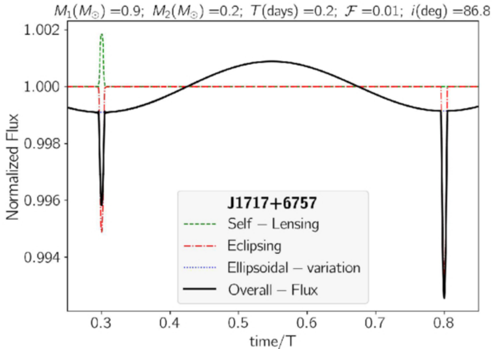
Figure 6. from Sedighe Sajadian and Aref Asadi 2025 Astron. J. 170 doi:10.3847/1538-3881/adf0f6 https://dx.doi.org/10.3847/1538-3881/adf0f6 © 2025. The Author(s). Published by the American Astronomical Society.
