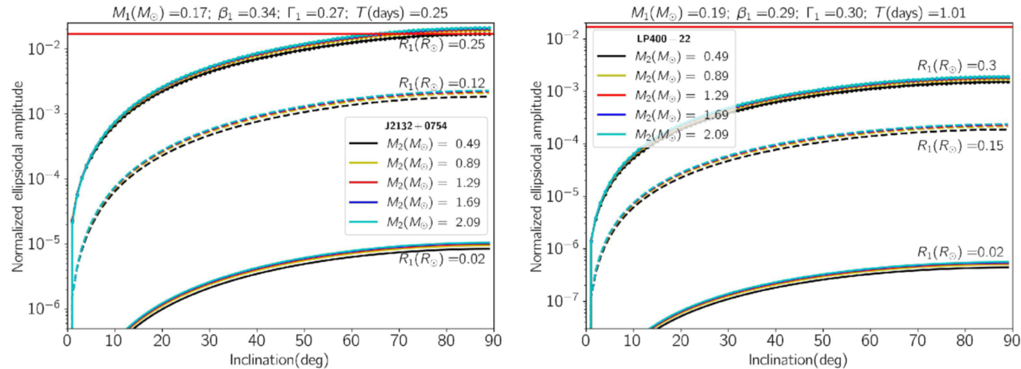
Figure 4. from Sedighe Sajadian and Aref Asadi 2025 Astron. J. 170 doi:10.3847/1538-3881/adf0f6 https://dx.doi.org/10.3847/1538-3881/adf0f6 © 2025. The Author(s). Published by the American Astronomical Society.
