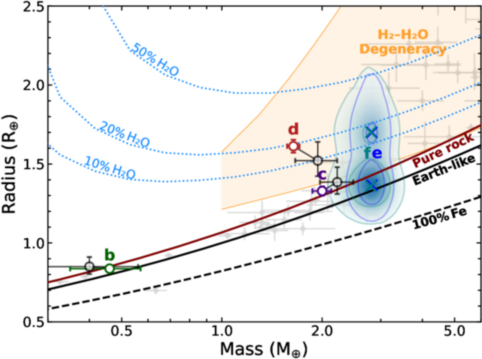
Figure 7. from Charles Cadieux et al 2025 Astron. J. 170 doi:10.3847/1538-3881/ade59 https://dx.doi.org/10.3847/1538-3881/ade59 © 2025. The Author(s). Published by the American Astronomical Society.
