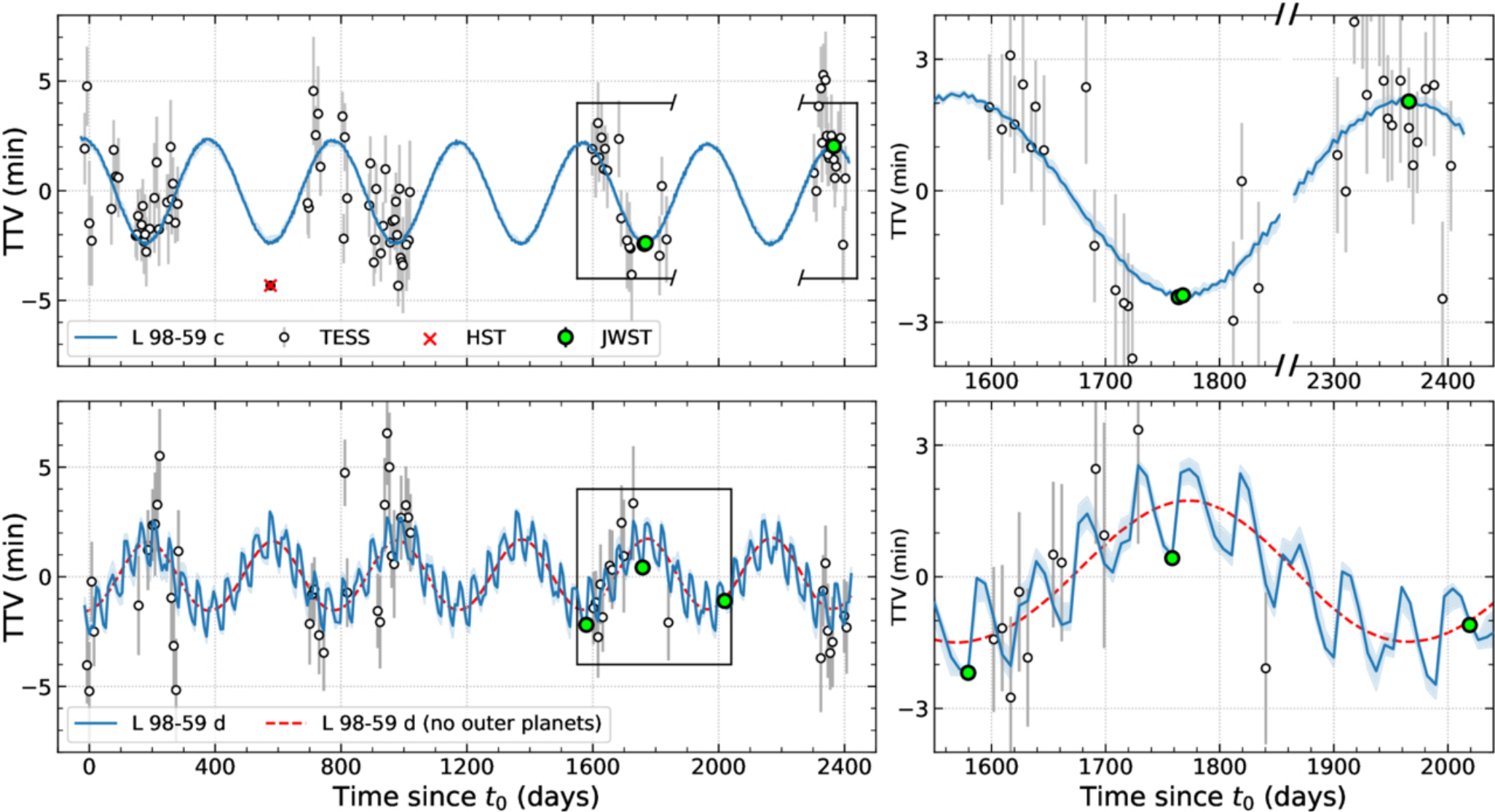
Figure 5. from Charles Cadieux et al 2025 Astron. J. 170 doi:10.3847/1538-3881/ade5f9 https://dx.doi.org/10.3847/1538-3881/ade5f9 © 2025. The Author(s). Published by the American Astronomical Society.
