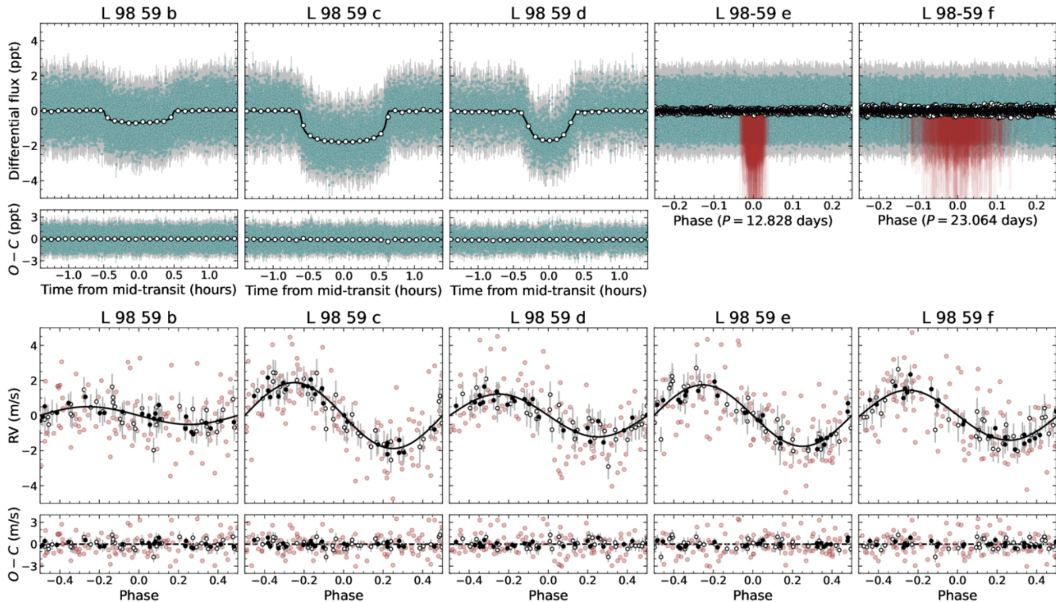
Figure 2. from Charles Cadieux et al 2025 Astron. J. 170 doi:10.3847/1538-3881/ade5f9 https://dx.doi.org/10.3847/1538-3881/ade5f9 © 2025. The Author(s). Published by the American Astronomical Society.
