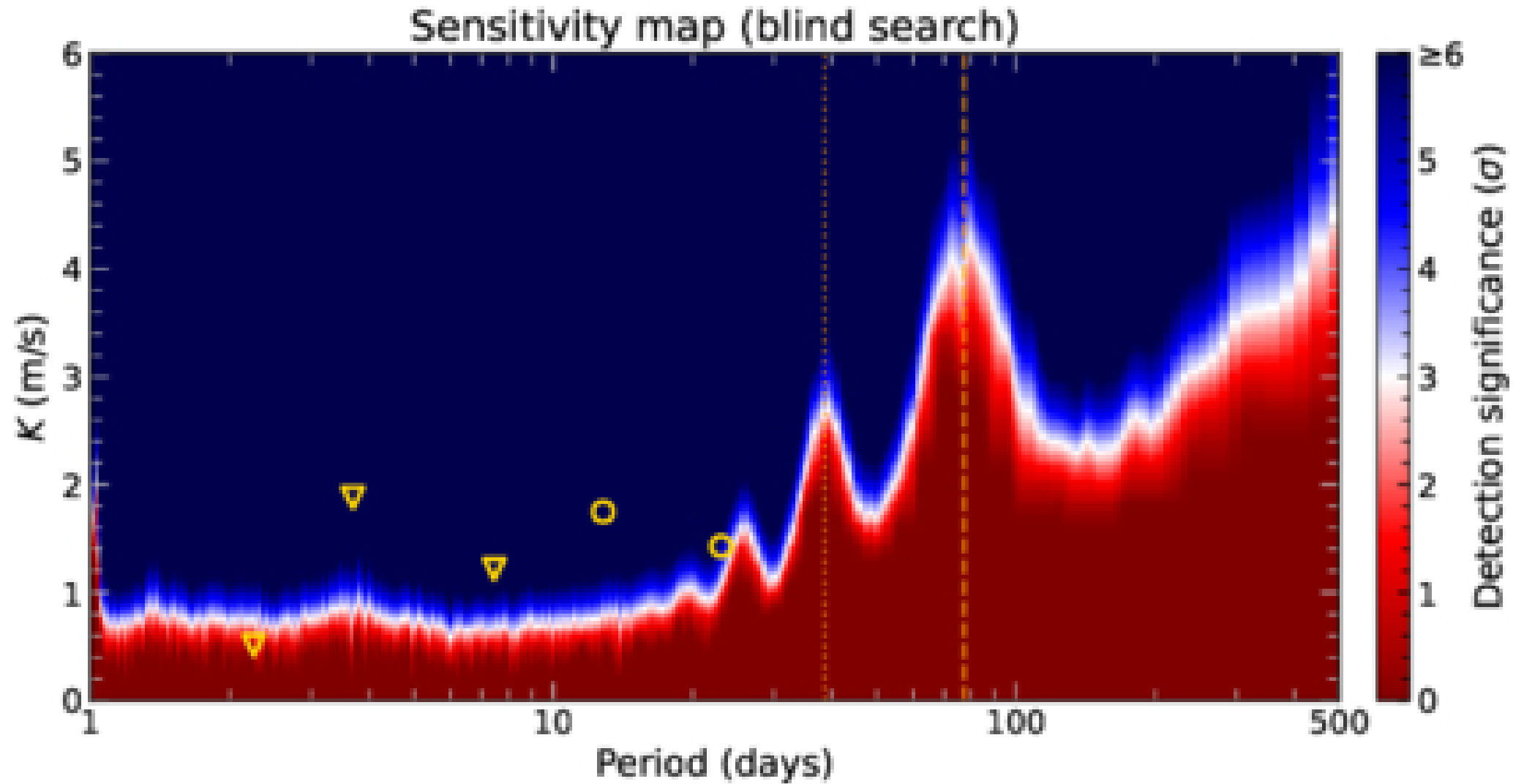
Figure C1. from Charles Cadieux et al 2025 Astron. J. 170 doi:10.3847/1538-3881/ade59 https://dx.doi.org/10.3847/1538-3881/ade59 © 2025. The Author(s). Published by the American Astronomical Society.
