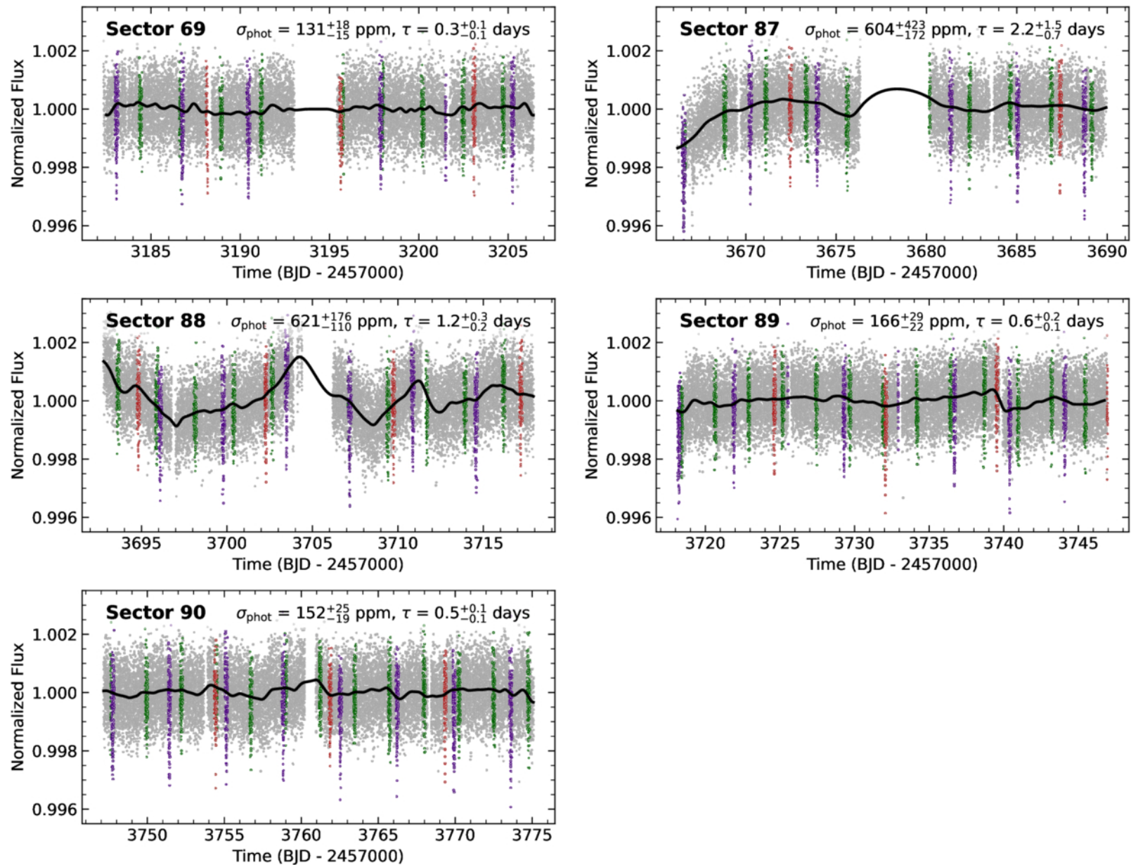
Figure A1. from Charles Cadieux et al 2025 Astron. J. 170 doi:10.3847/1538-3881/ade5f9 https://dx.doi.org/10.3847/1538-3881/ade5f9 © 2025. The Author(s). Published by the American Astronomical Society.
