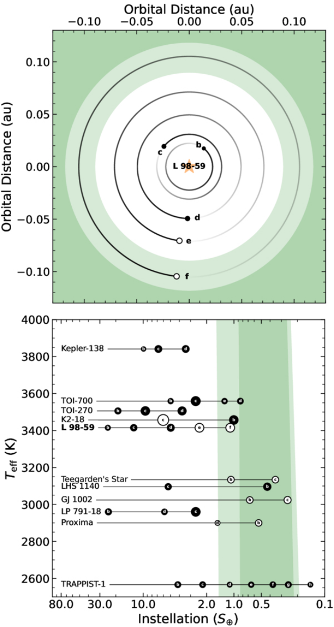
Figure 1. from Charles Cadieux et al 2025 Astron. J. 170 doi:10.3847/1538-3881/ade59 https://dx.doi.org/10.3847/1538-3881/ade59 © 2025. The Author(s). Published by the American Astronomical Society.
