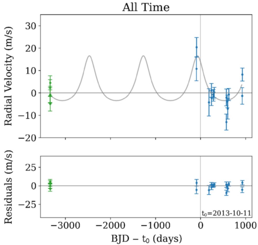
Figure 4. from Simone R. Hagey et al 2025 Astron. J. 170 doi:10.3847/1538-3881/aded15 https://dx.doi.org/10.3847/1538-3881/aded15 © 2025. The Author(s). Published by the American Astronomical Society.
