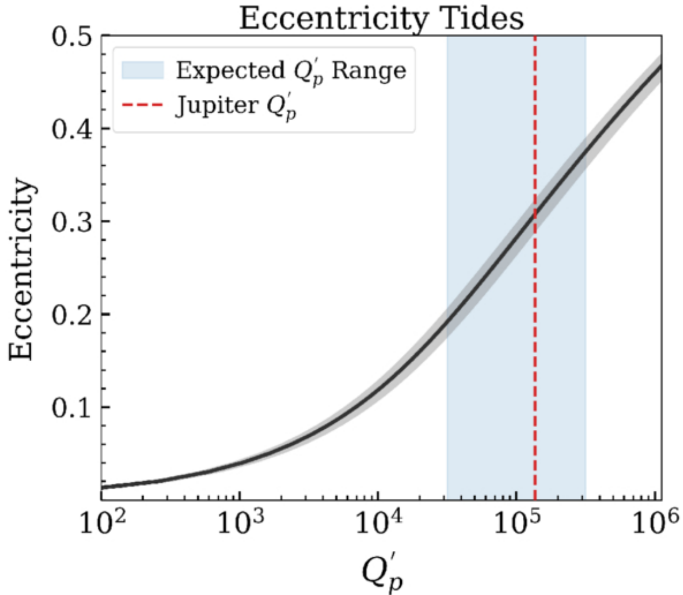
Figure 10. from Simone R. Hagey et al 2025 Astron. J. 170 doi:10.3847/1538-3881/aded15 https://dx.doi.org/10.3847/1538-3881/aded15 © 2025. The Author(s). Published by the American Astronomical Society.
